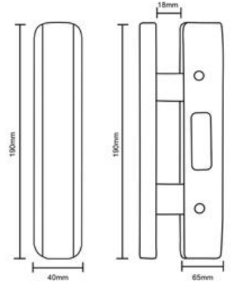
Strike Dimension
