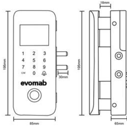
Body Dimension
