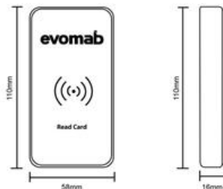
Sensor Dimension
