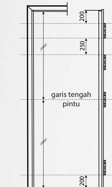
2400 ~ 2700mm (4 Engsel)
