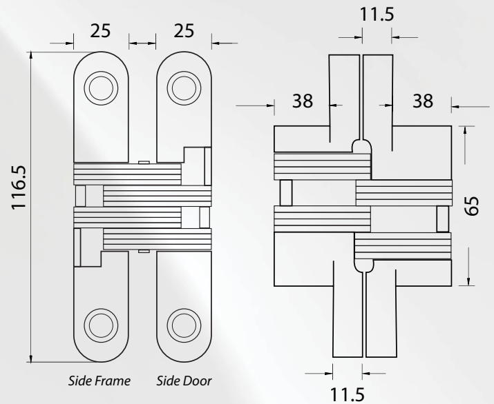
Gambar Bobokan Invisible Hinge (mm)
