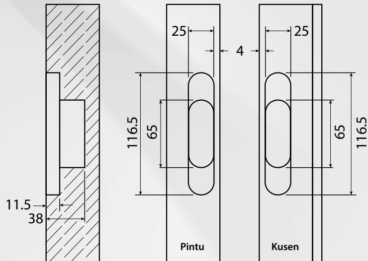
Gambar Bobokan Invisible Hinge (mm)
