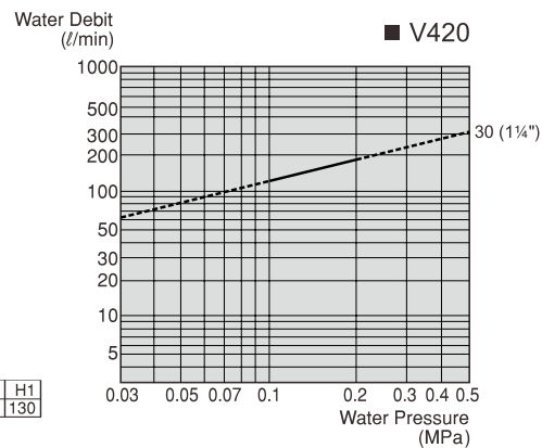
Water Debit VS Pressure
